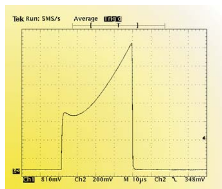
A 2700A current pulse with a 6700A/ \mu s falling edge measured by a CWT15 with a 500mm coil and a very high bandwidth coaxial shunt - 10/ \mu s/div.
